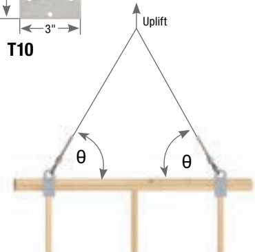
Typical 60° installation
