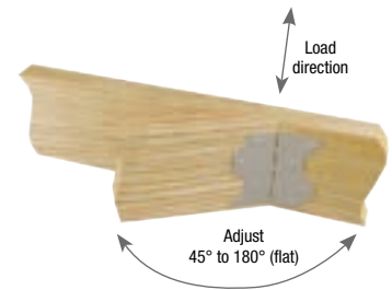
Typical MP joist / header installation
