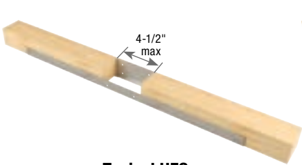
Typical HFS installation to underside of double top plates.
