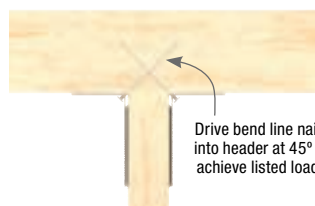
Typical bend line nailing installation
