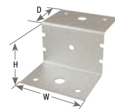
ZC2
