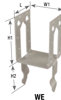
Typical WE installation
