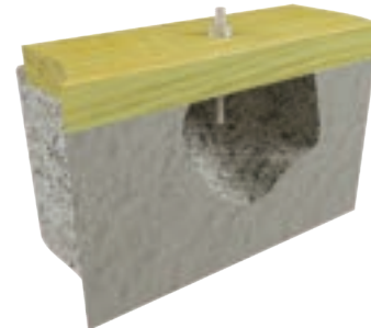
Typical THR installation
