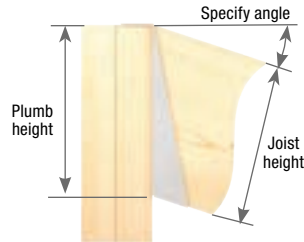
Typical BPHA hanger sloped seat, down shown
