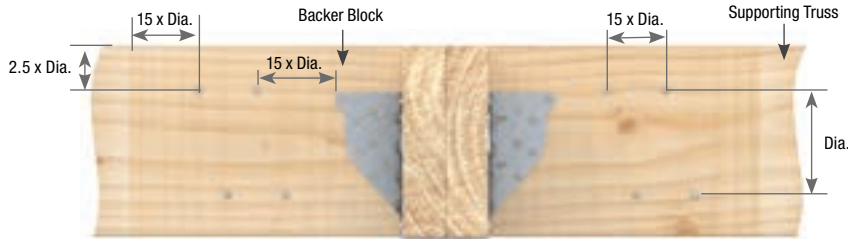
Nail Backer Block Distances
