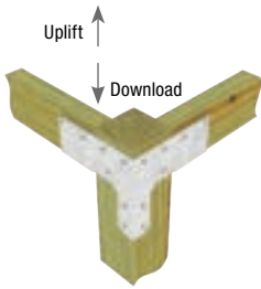
Typical TTC42-TZ installation
