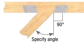
Typical BPHA hanger skewed, left shown (bevel cut)
