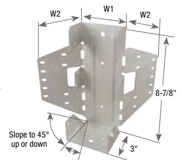
LSSH35-TZ
