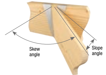
Typical BPHA hanger sloped down, skewed right, high side flush shown
