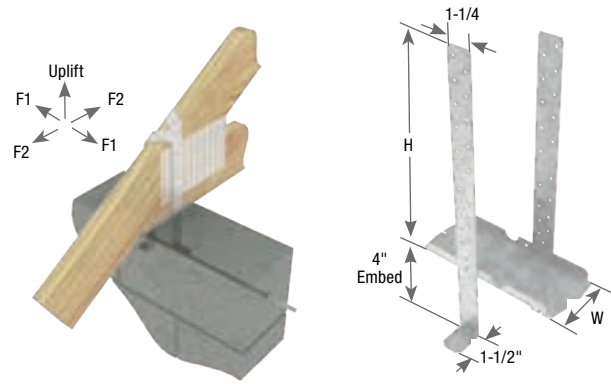
Typical DHTA 1-Ply installation
