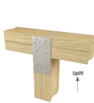
Typical RSPT6-2 installation
