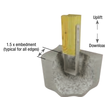
Typical CBE installation
