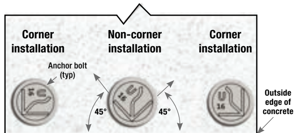
Plan view of STB/STBL placement in concrete stemwall
