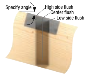
Typical BPHA hanger sloped down top flange right shown (this configuration will not be open back)
