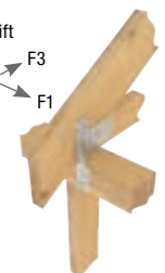
Typical TSP truss/rafter installation (max nailing)
