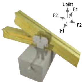
Typical HLPTA75 double anchor installation
