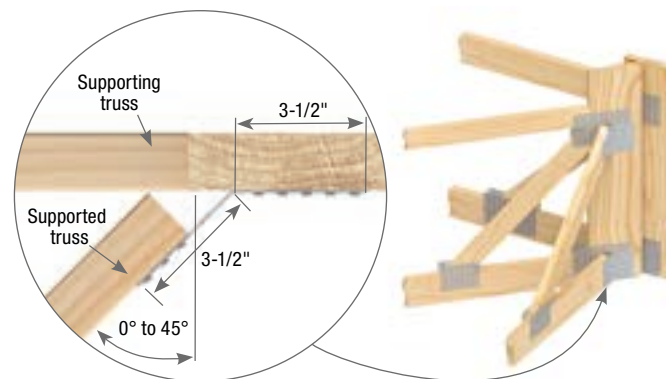
Alternate SNP installation
