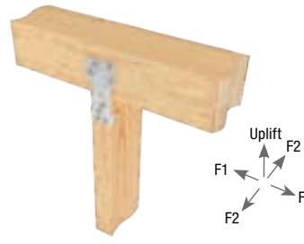
Typical RSPT4 double plate installation
