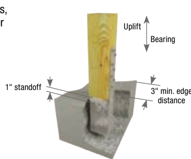
Typical CBSQ installation
