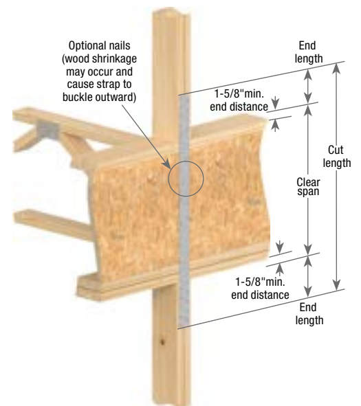
Typical KST237 floor-to-floor installation
