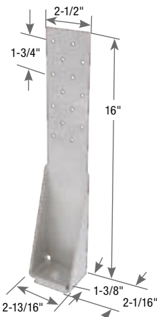
HTT14S
