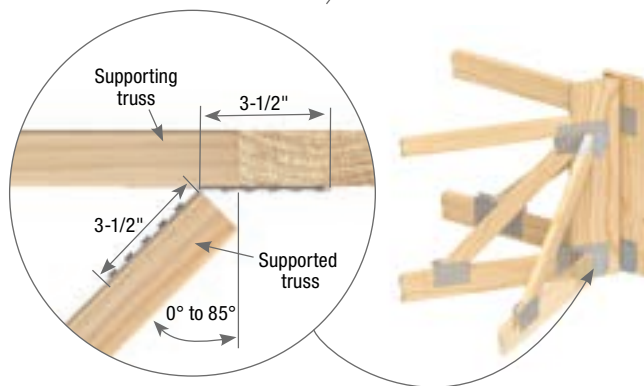
Standard SNP installation
