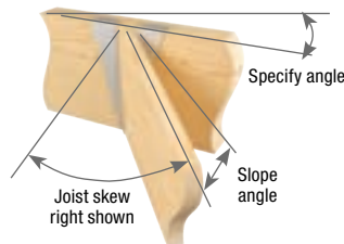
Typical BPHA hanger skewed right, sloped down, top flange sloped
