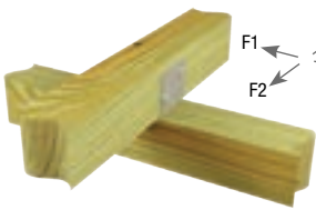
Typical TTU2-TZ installation
