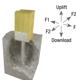
Typical EPB installation
