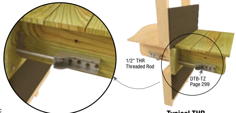
Typical THR deck to ledger installation
