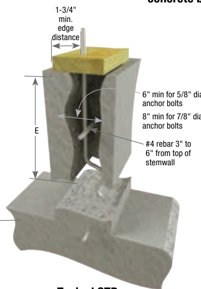
Typical STB anchor bolt installation
