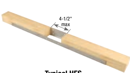
Typical HFS installation to underside of double top plates.
