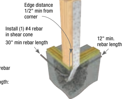
Typical STAD10 corner installation
