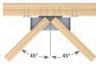
Typical HHC installation top view
