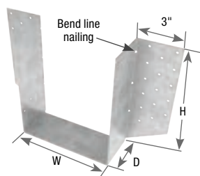
THD7210
