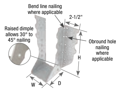
THDH
