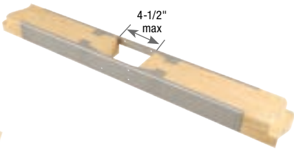
For wall depth larger than 3-1/2", separate HFS into two pieces (L shape)
